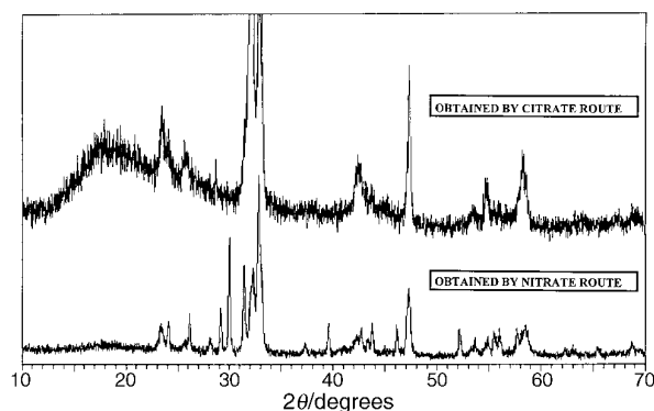
Fig. 3 X-Ray powder diffraction patterns of the precursor of \text{La}_3\text{Ni}_2\text{O}_{7-\delta} after heating for 2 h at 1173 K
