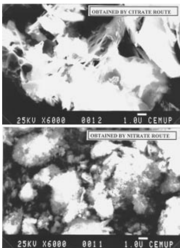
Fig. 2 SEM images of the precursor of \text{La}_4\text{Ni}_3\text{O}_{10-\delta}
