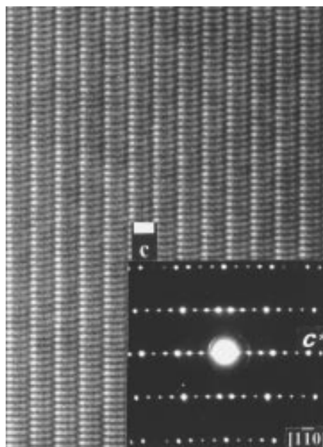
Fig. 8 High resolution electron microscopy image of \text{La}_4\text{Ni}_3\text{O}_{10-\delta} (citrate route) ( [110] zone axis)
