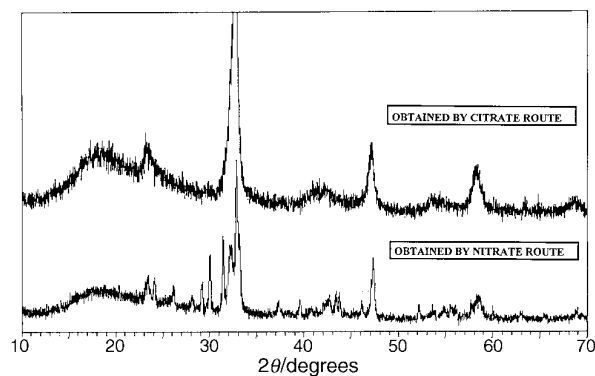
Fig. 4 X-Ray powder diffraction patterns of the precursor of \text{La}_4\text{Ni}_3\text{O}_{10-\delta} after heating for 2 h at 1173 K
